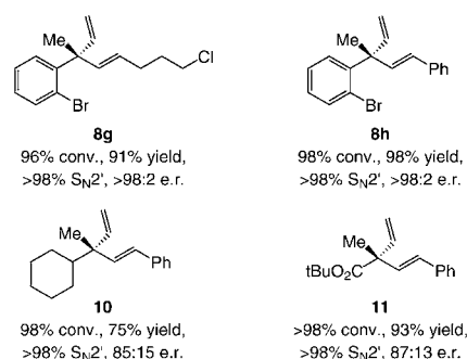
Scheme 2. Products of NHC–Cu-catalyzed EAS of various trisubstituted allylic phosphates and different readily accessible vinylboron reagents. All reactions were performed with 5.5 mol % 6b ; see Table 2 for conditions and the Supporting Information for details.
