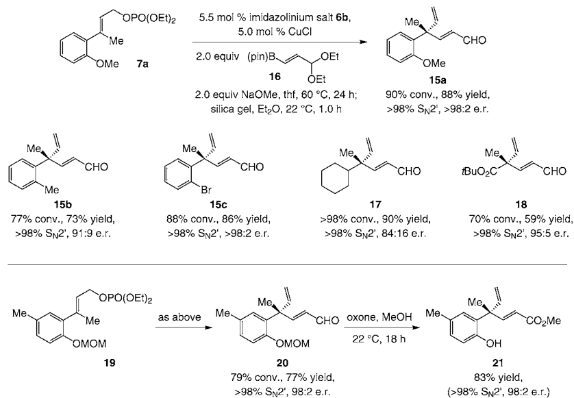
Scheme 4. NHC–Cu-catalyzed EAS of allylic phosphates with acetal-containing alkenylboron compound 16 .
