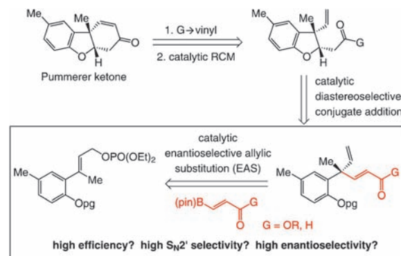
Scheme 1. A route for enantioselective synthesis of Pummerer ketone might involve catalytic allylic substitution with a carbonyl-containing vinyl group, followed by a catalytic diastereoselective intramolecular conjugate addition and catalytic ring-closing metathesis. pg = protecting group, pin = pinacolato.
