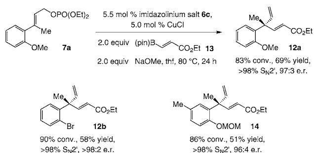
Scheme 3. NHC–Cu-catalyzed EAS with allylic phosphates and carboxylic ester containing vinylboron 13 . MOM = methoxymethyl.
